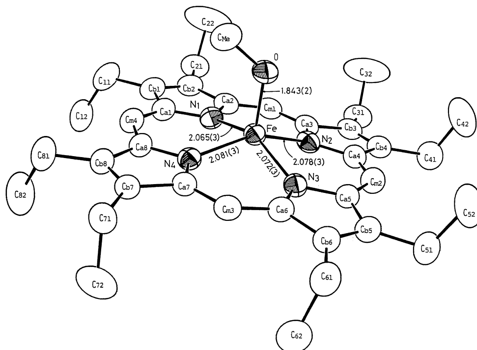
Fig. 1. ORTEP diagram(Johnson, 1976) and labeling scheme for all non-hydrogen atoms of the \text{Fe}(\text{OEP})(\text{OMe}) molecule. Bond lengths of the coordination sphere of iron are entered in units of Å.
