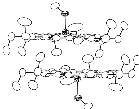
Fig. 2. An overall view of the \pi - \pi dimer in the lattice of \text{Fe}(\text{OEP})(\text{OMe}) . The porphinato planes are approximately perpendicular to the plane of the plot.
